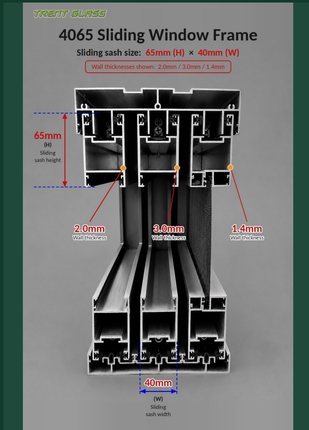
4065 section: 65 x 40 mm sliding sash
